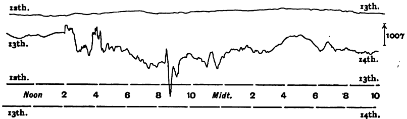
FIG. 3.—KEW HORIZONTAL FORCE. NOVEMBER 12-14, 1894.
